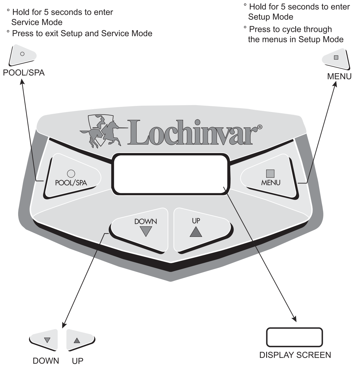
Figure 3-1_ Control Panel
