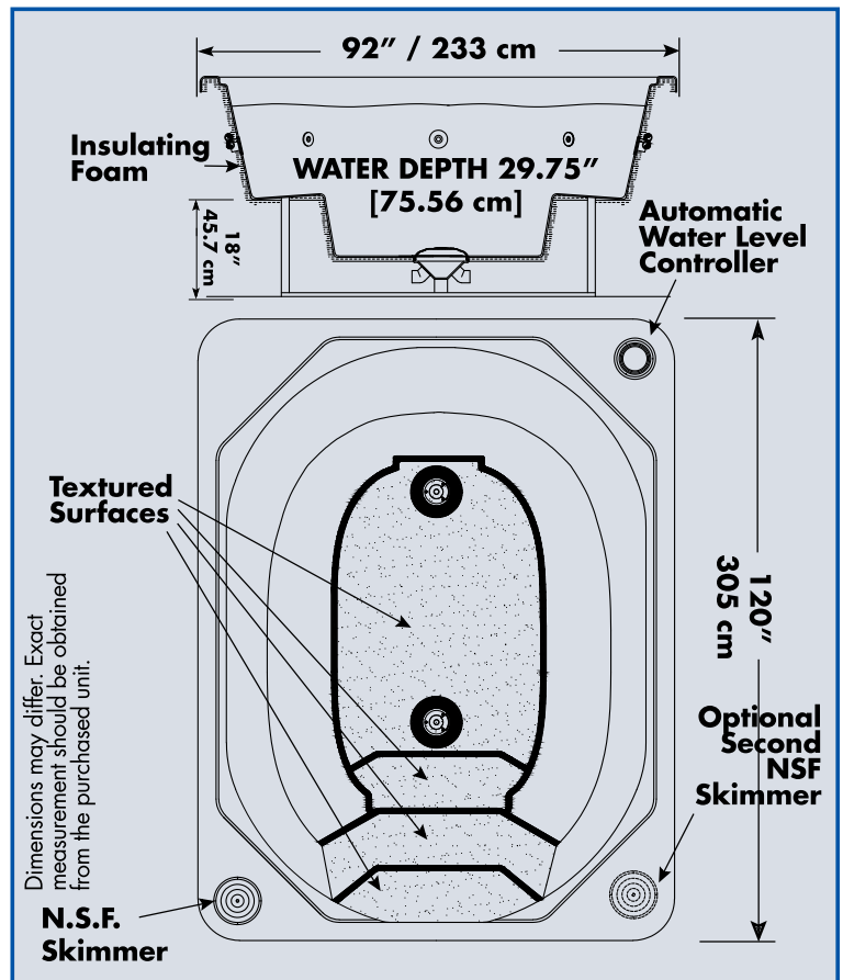
Technical drawing showing dimensions and features of the hot tub, including water depth, overall height, and width.
