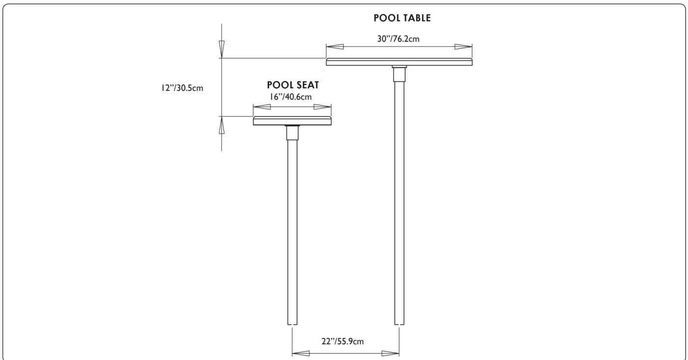
Figure 8: Pool/Spa Table & Seat Recommended Placement Diagram
