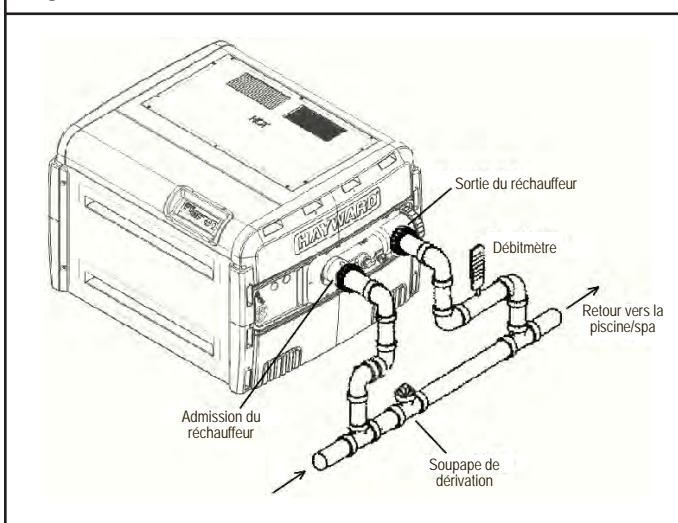
Figure 16: Soupape de dérivation manuelle
