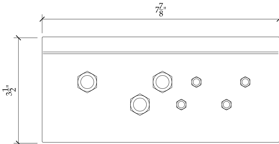
BOTTOM VIEW
