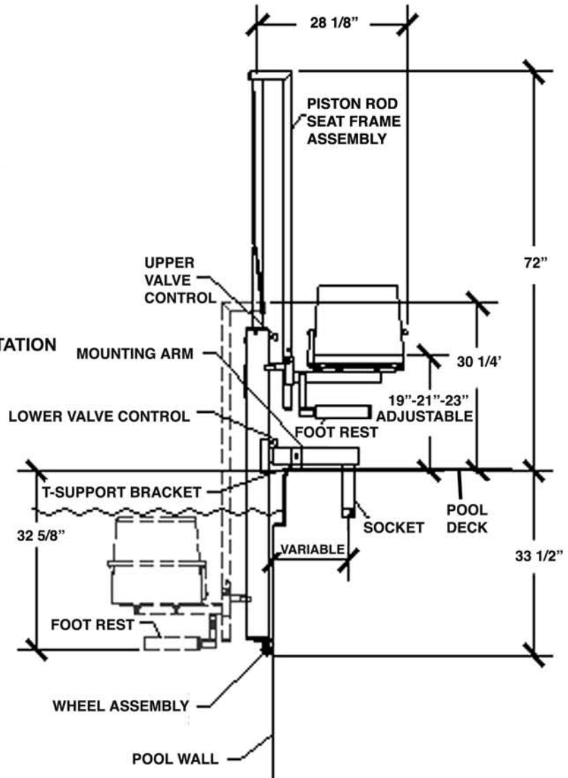
SIDE VIEW MODEL IGAT-180/135 STANDARD ROTATION
